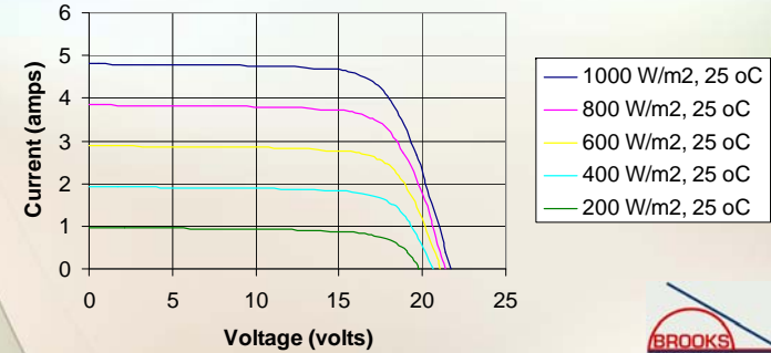
Siemens Solar Module SP75 Performance at Different Irradiances
